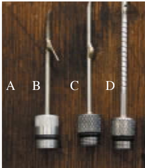
Assortment of dart needles for rhino work
